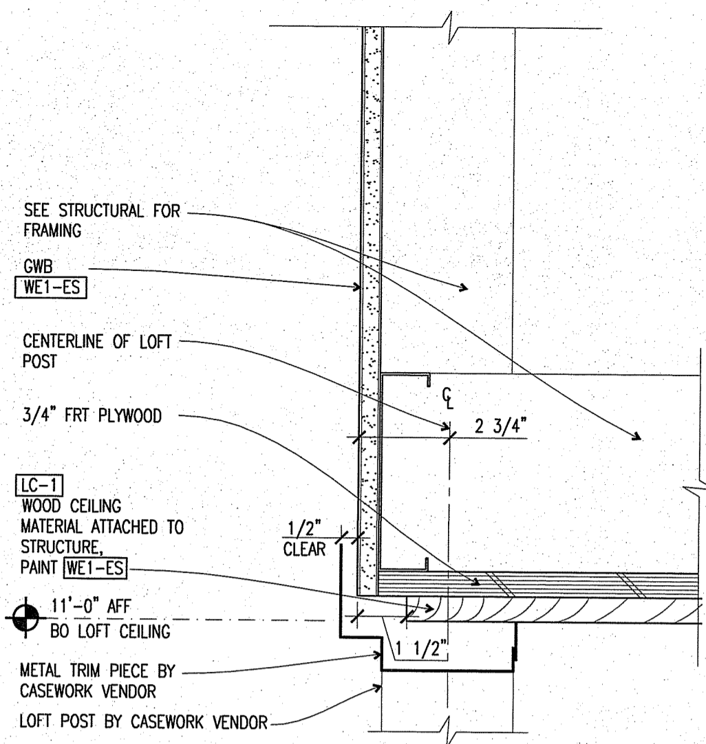
E1 SECTION @ LOFT SOFFIT 3'-1'-0"
