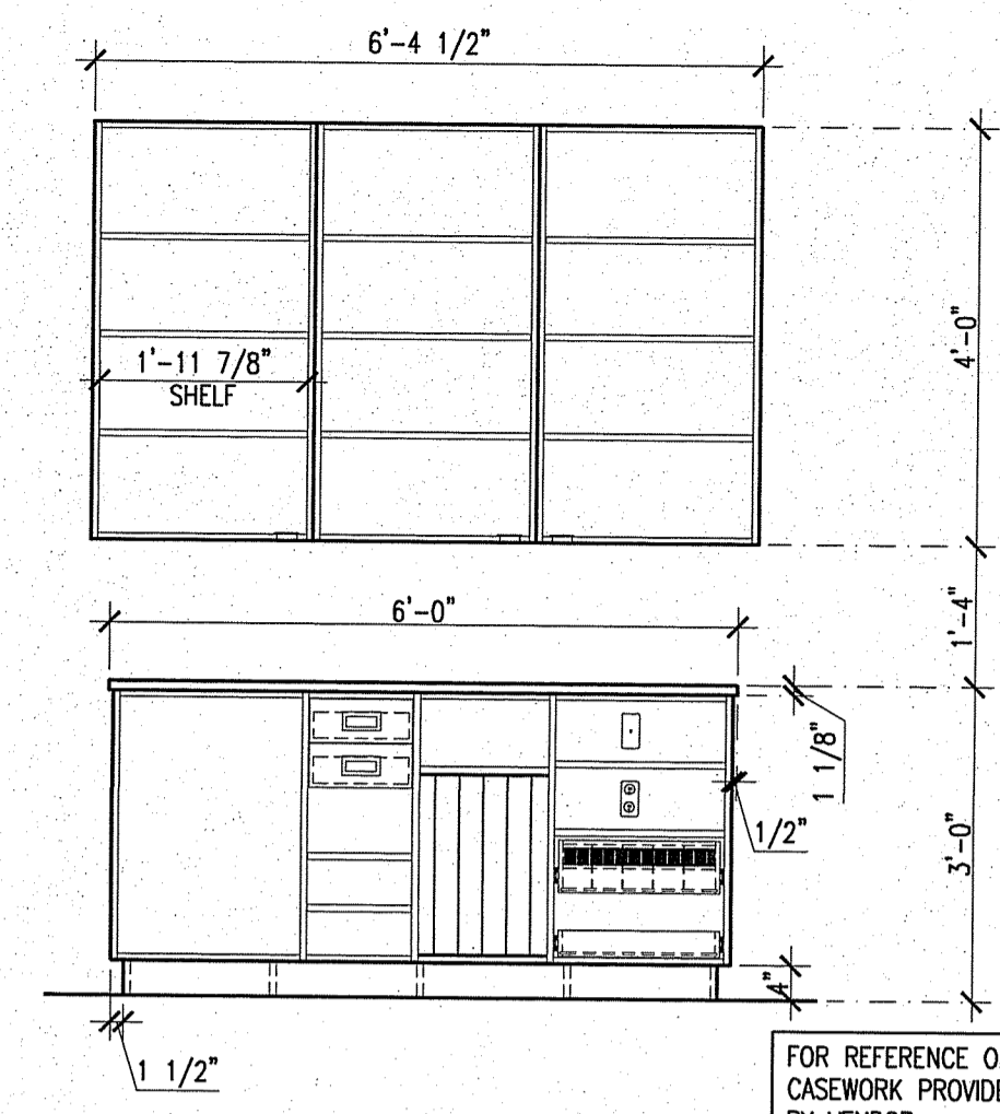
E7 CUSTOMER SERVICE COUNTER 1/2"=1'-0"
