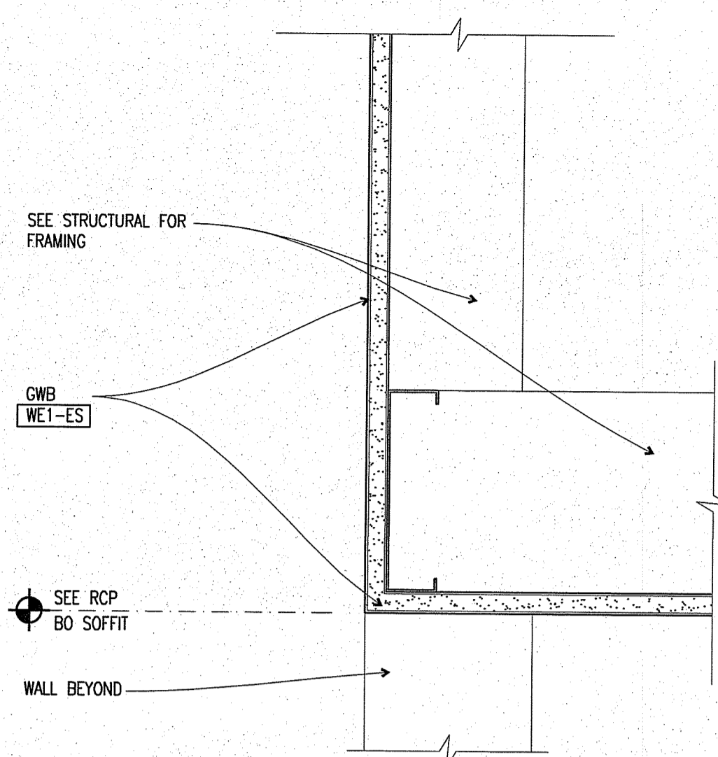
E2 SOFFIT @ BACK OF HOUSE 3'-1'-0"
