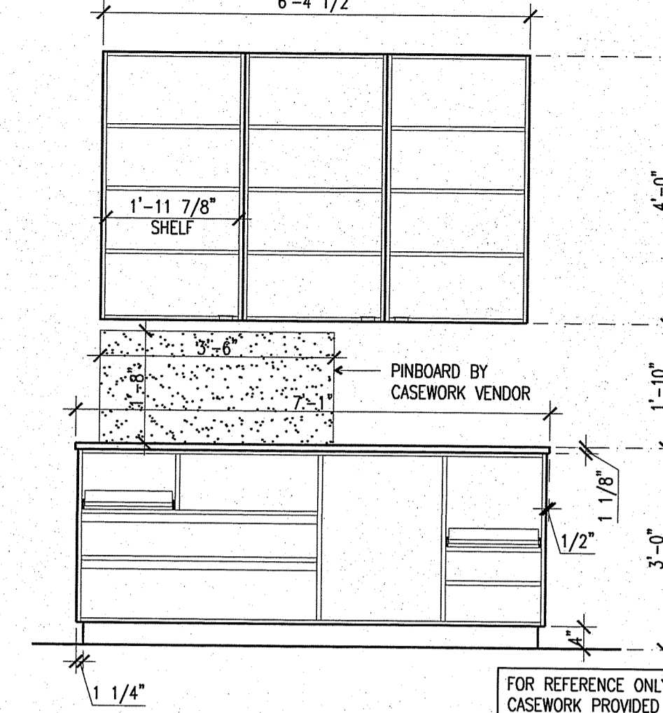
E9 SHIPPING/RECEIVING COUNTER 1/2"=1'-0"
