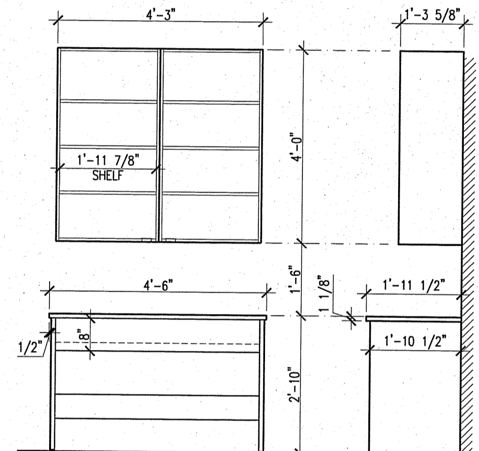
C9 EMPLOYEE COUNTER 1/2"=1'-0"
