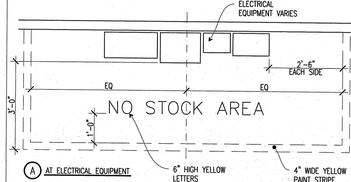
A9 CLEAR AREA STRIPING 1/2"=1'-0"
